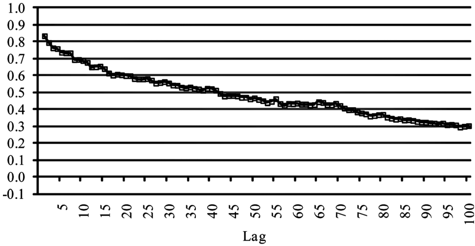
ACF for FDAX Realized Variance 1/3/2000 - 5/15/2012
